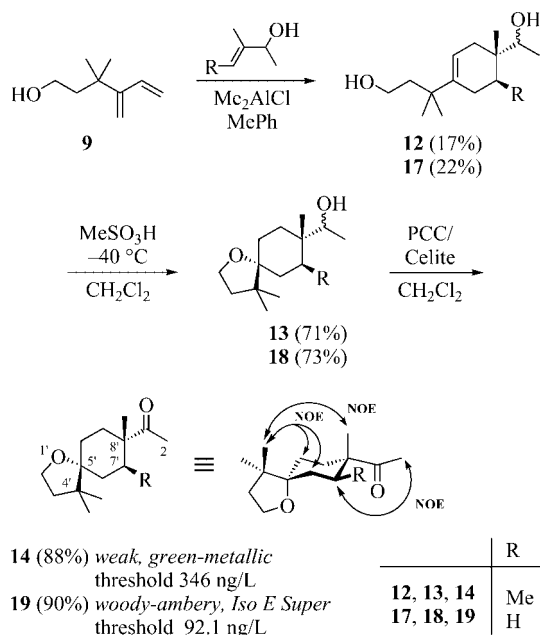
Scheme 2. Synthesis of the para -configured 8-acetyl-substituted target compounds 14 and 19 by Diels–Alder reaction with (3 E )-3-methylpent-3-en-2-ol and 3-methylbut-3-en-2-ol.
