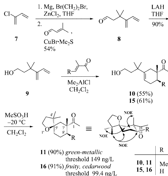
Scheme 1. Synthesis of undesired meta -configured 7-acetyl-4,4-dimethyl-1-oxaspiro[4.5]decanes 11 and 16 by an aluminum-tethered Diels–Alder reaction.
