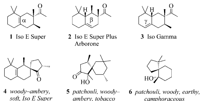
Figure 1. The woody–ambery benchmark odorants 1 – 3 , the powerful soft, woody–ambery spirocyclic ketone 4 , and two intense patchouli-like, woody spirocycles 5 and 6 .
