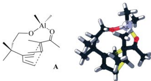
Figure 2. Proposed 10-membered transition state A for the Diels–Alder reaction of the dihomomallylic dienol 9 and ( E )-3-methylpent-3-en-2-one, tethered by dimethylaluminum chloride.
